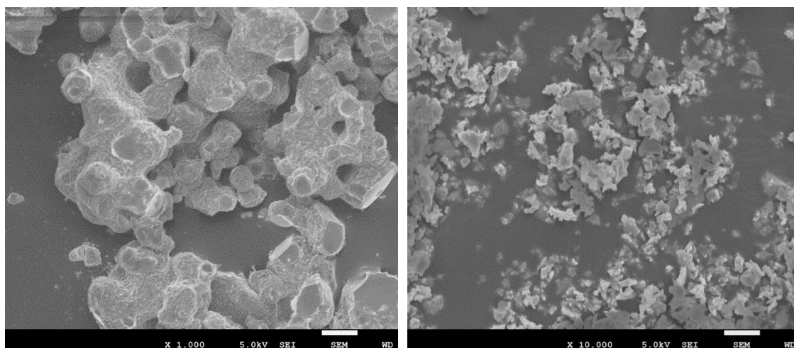
SEM Observation of synthesized Ga-LLZO left : several \mu\text{m} , right 300-500 nm
